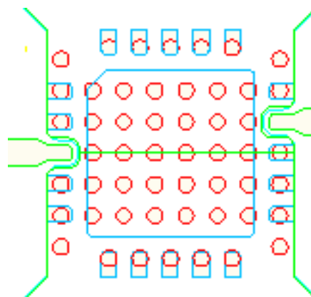
MOUNTING PATTERN
