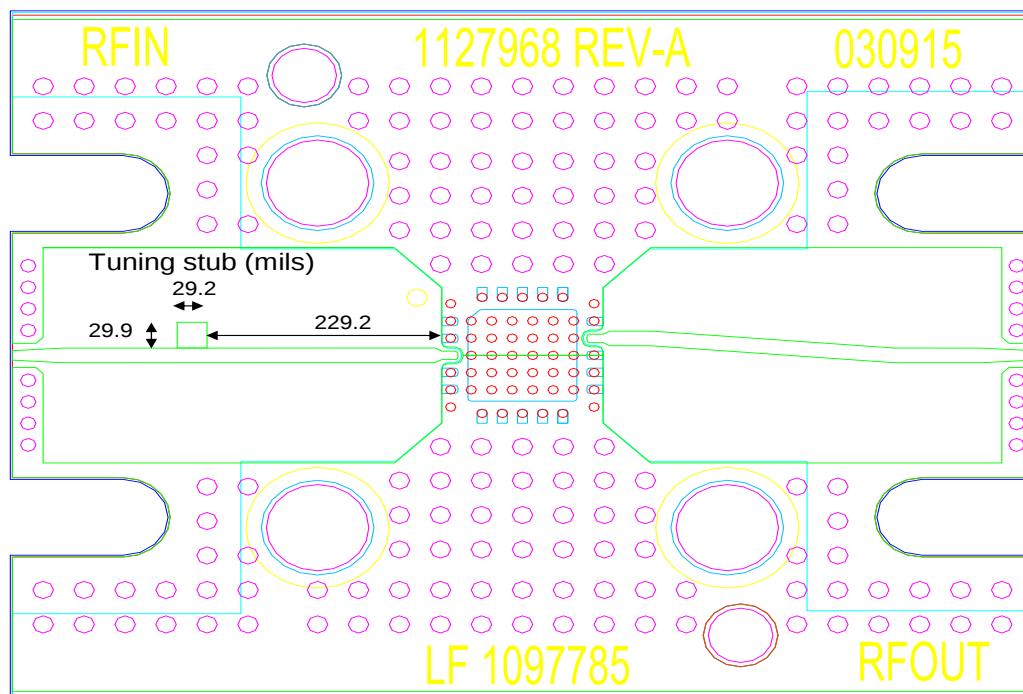
TUNED PCB LAYOUT
