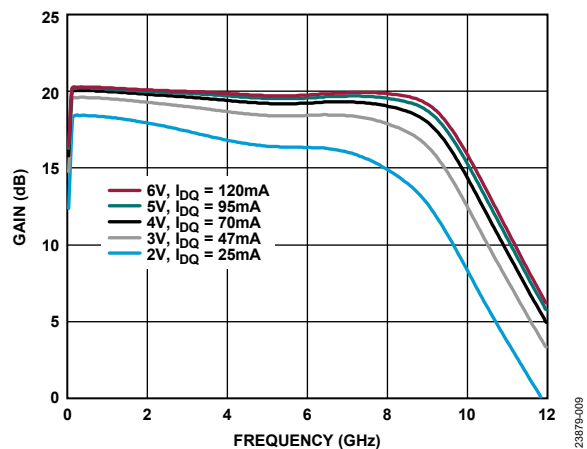
Figure 9. Gain vs. Frequency for Various Supply Voltages and I_{DQ} , R_{BIAS} = 787\text{ }\Omega
