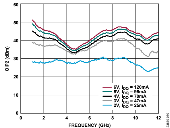
Figure 60. OIP2 vs. Frequency for Various Supply Voltages and I_{DQ} , 1 GHz to 12 GHz, R_{BIAS} = 787 Ω
