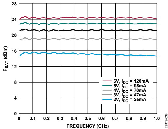
Figure 38. P_{SAT} vs. Frequency for Various Supply Voltages and I_{DQ} , 0.01 GHz to 1.0 GHz, R_{BIAS} = 787\text{ }\Omega
