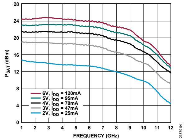
Figure 41. P_{SAT} vs. Frequency for Various Supply Voltages and I_{DQ} , 1 GHz to 12 GHz, R_{BIAS} = 787\text{ }\Omega
