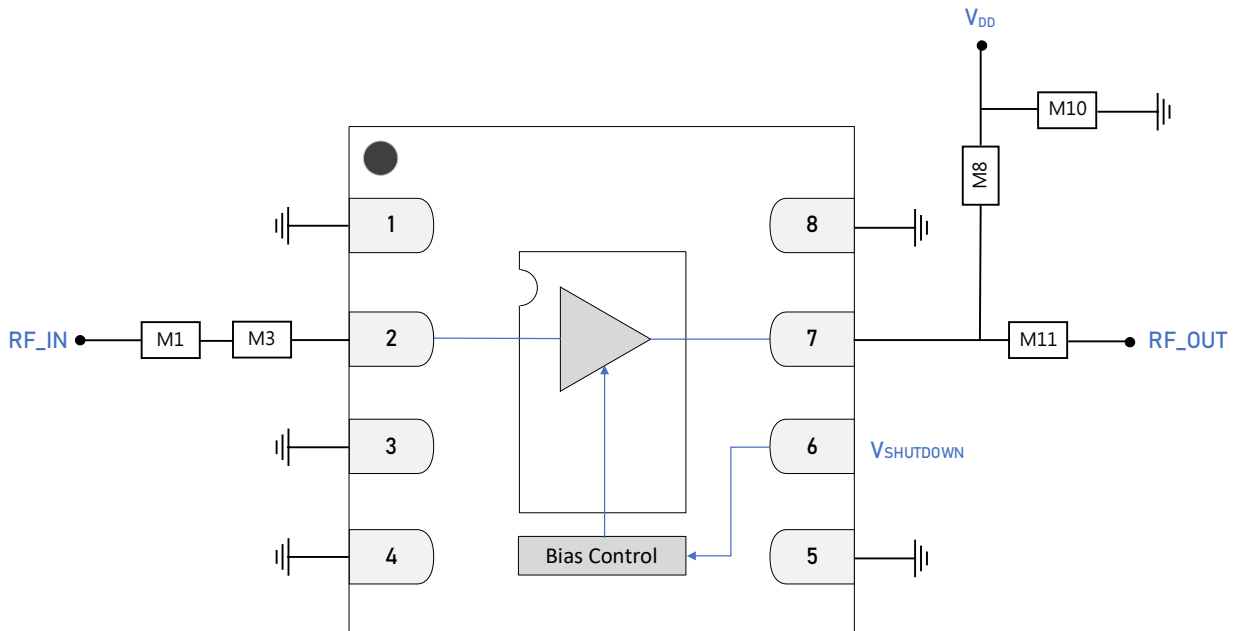
GRF2080 Standard Test Schematic
