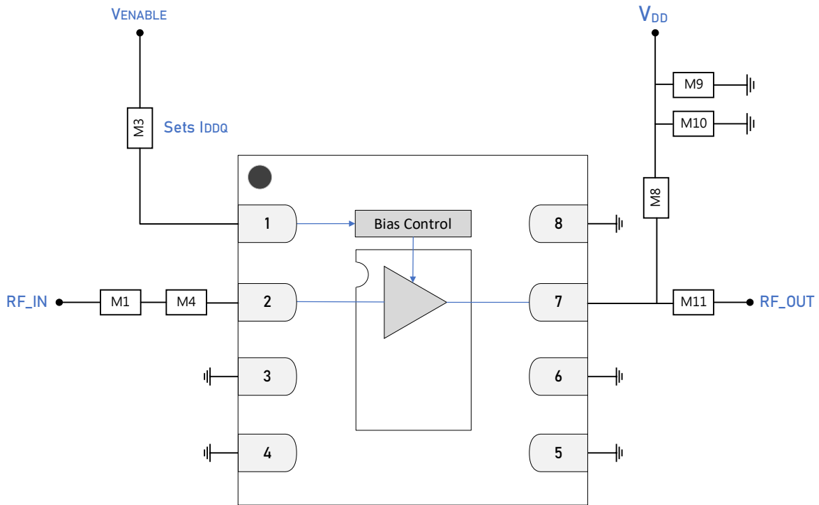
GRF2073 Standard Test Schematic
