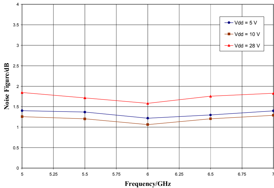
Noise Figure vs. V_{dd} , I_{dd} = 200\text{ mA} , T_A = 25\text{ °C}
