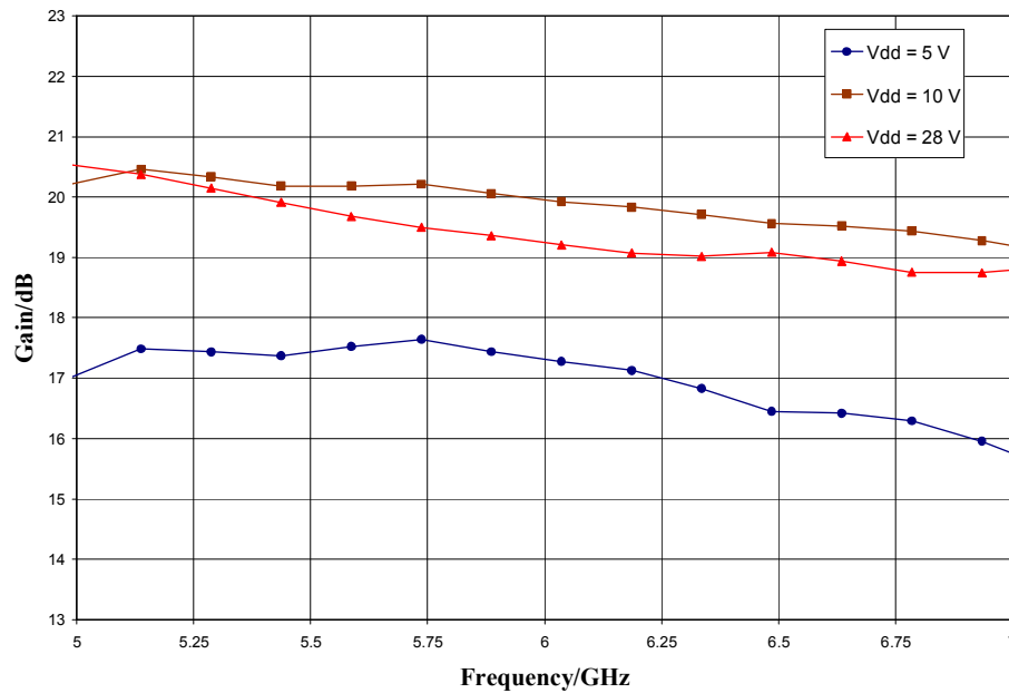
Gain vs. V_{dd} , I_{dd} = 200\text{ mA} , T_A = 25\text{ °C}
